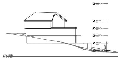
North 1:100
