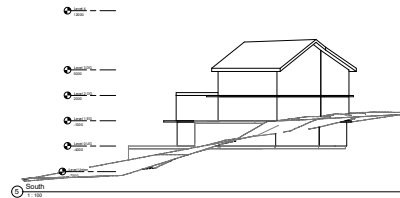
South 1:100
