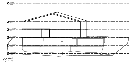
West 1:100
