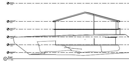
East 1:100
