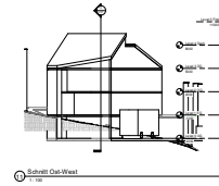
Section East-West
