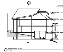
Section East-West
