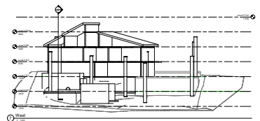
Section 3 (West)
