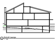
Section 1 (East)
