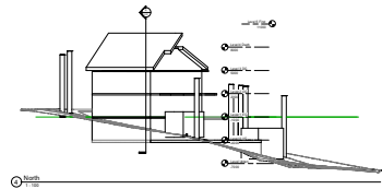
Section 7 (North)
