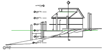
Section 6 (South)
