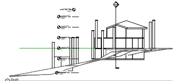
Section 6 (South) 1:100
